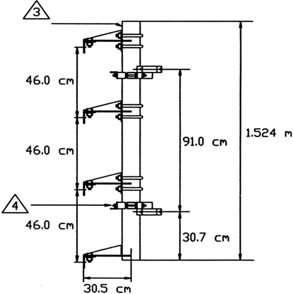
ANTENNA PIPE MOUNT
